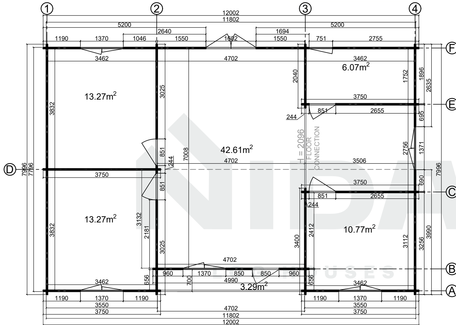
Floor plan
