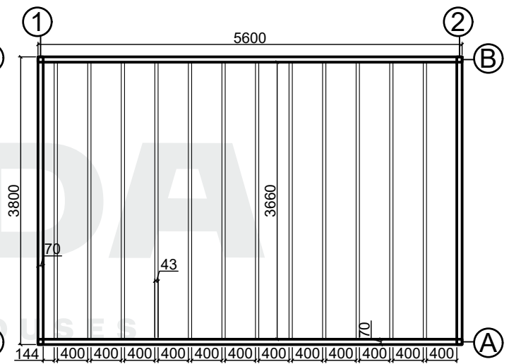
Base plan
