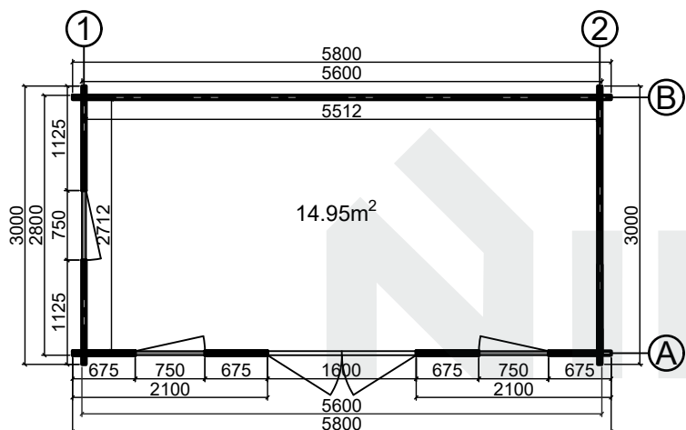
Floor plan
