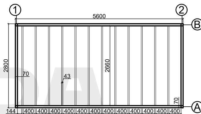
Base plan
