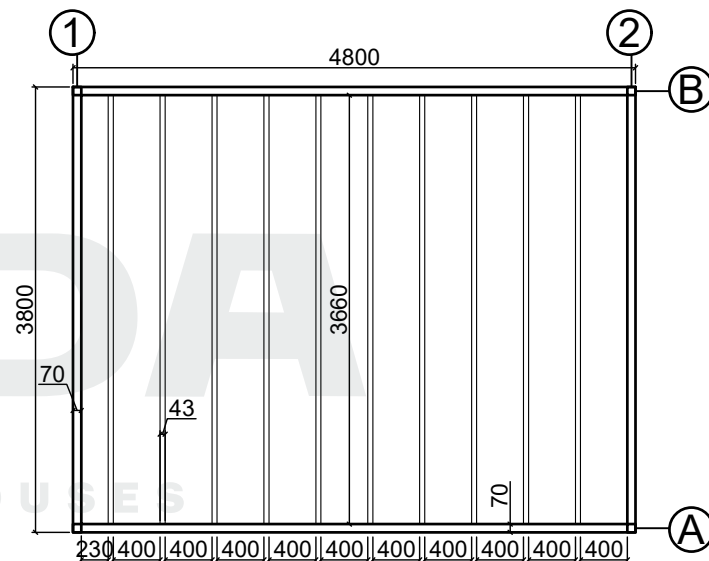
Base plan
