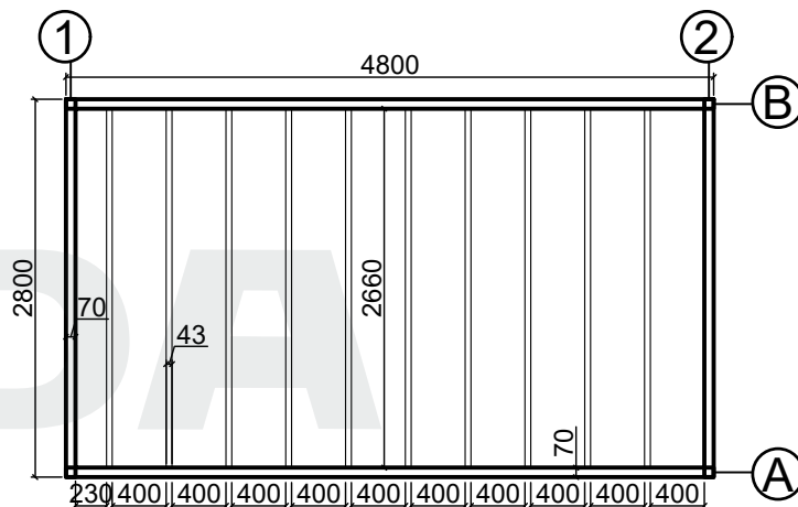
Base plan
