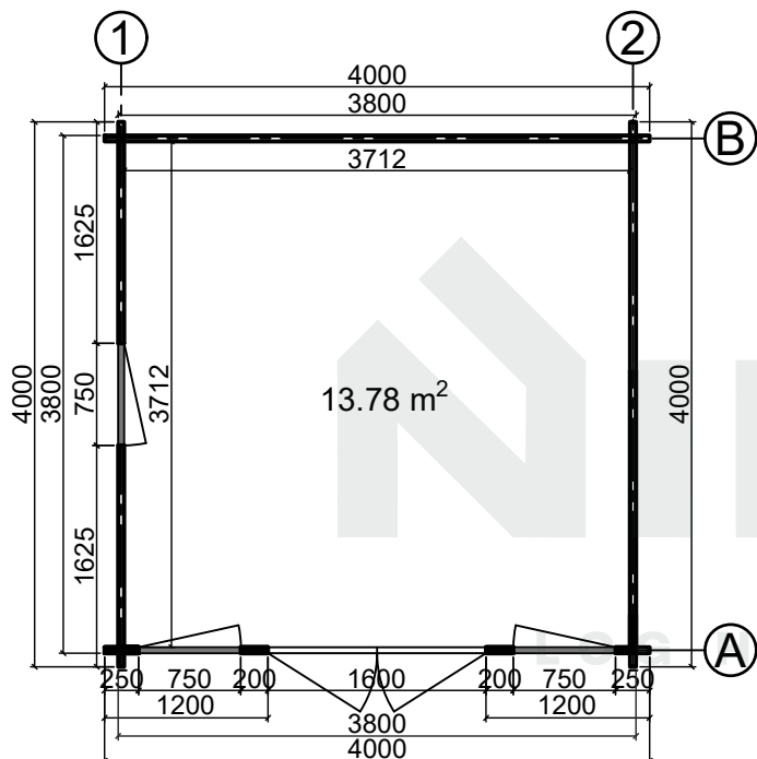
Floor plan
