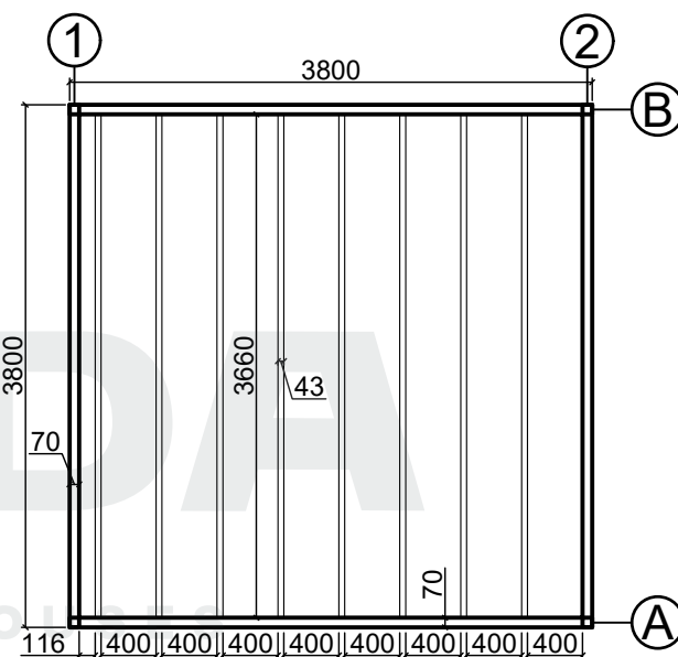
Base plan
