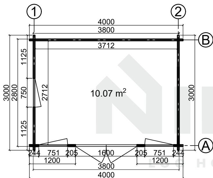
Floor plan
