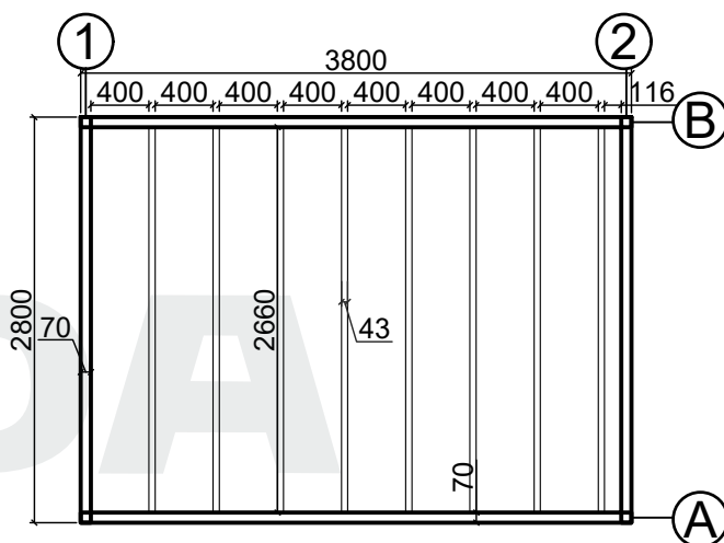
Base plan
