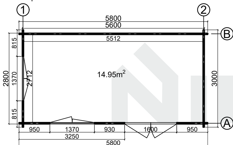
Floor plan
