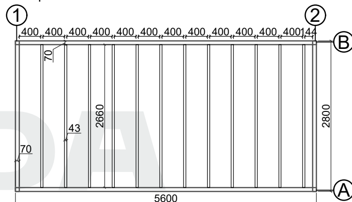
Base plan
