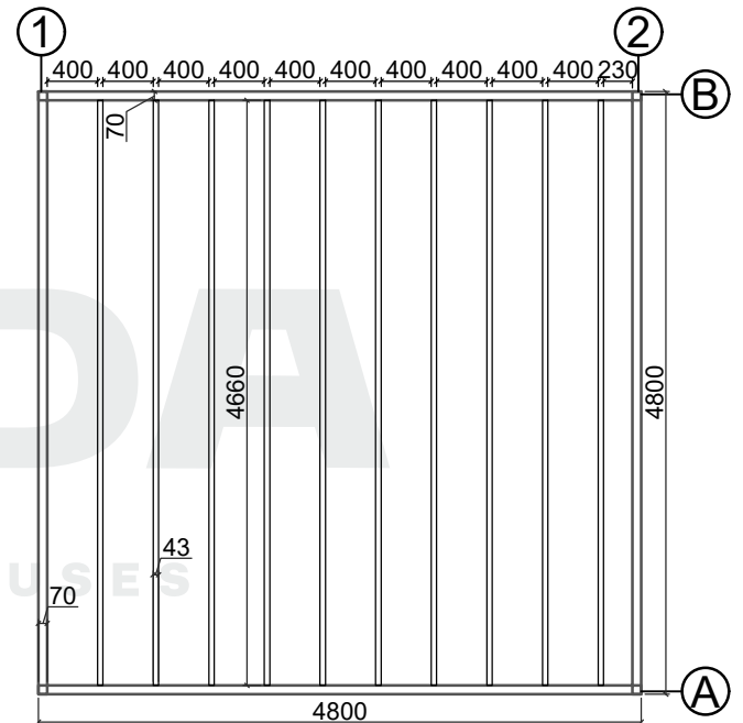
Base plan
