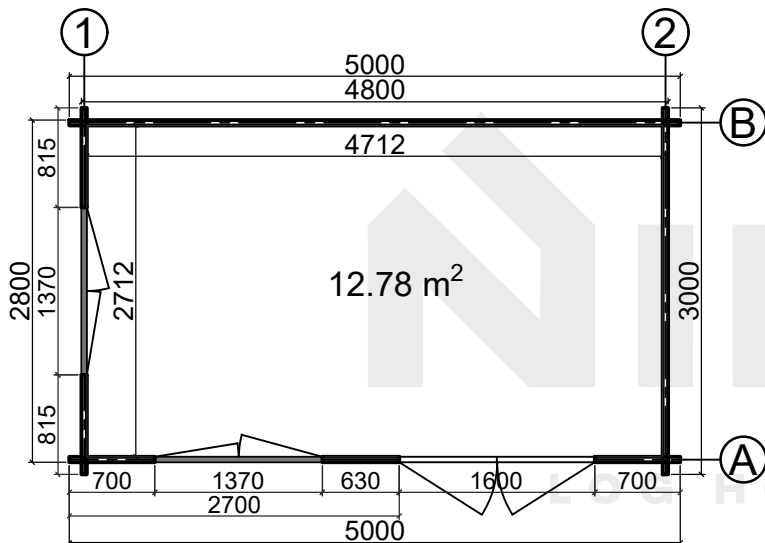
Floor plan
