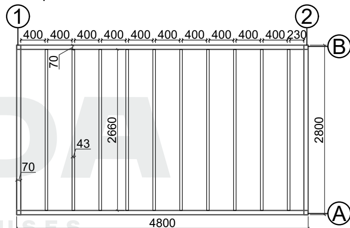
Base plan
