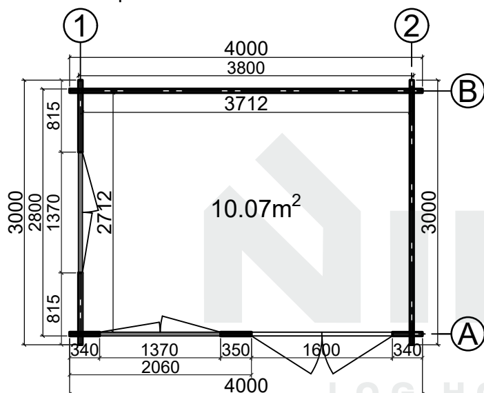
Floor plan
