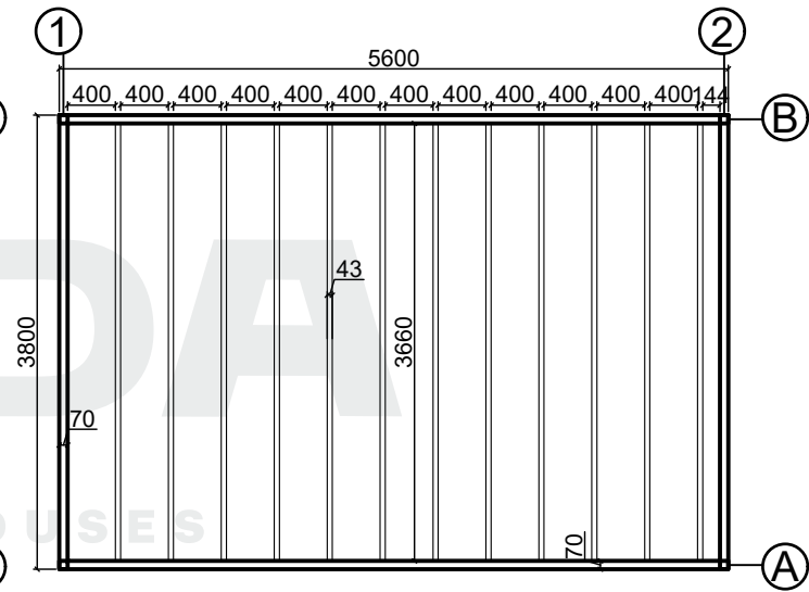
Base plan
