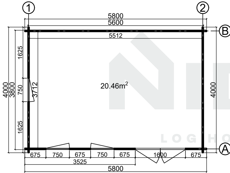
Floor plan
