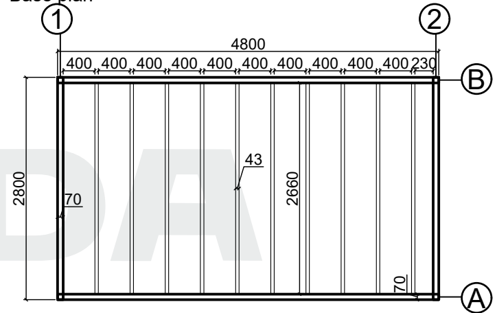
Base plan
