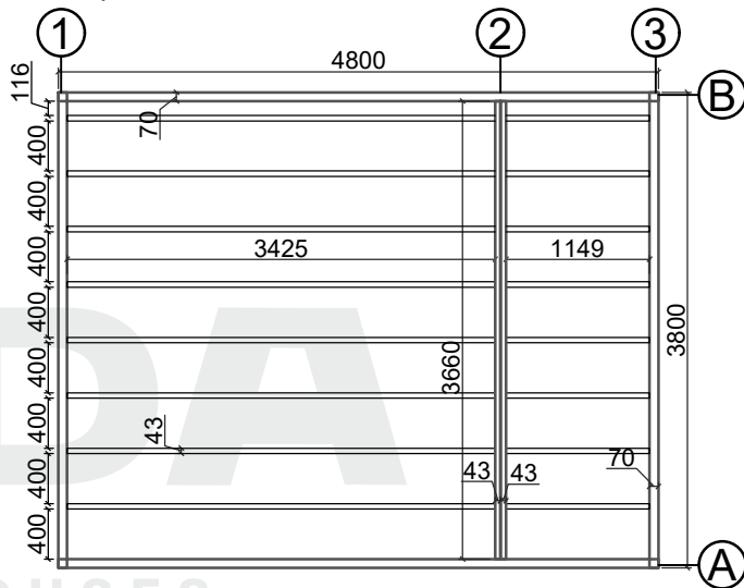
Base plan
