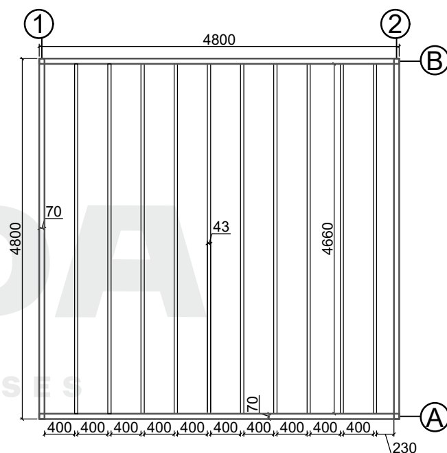
Axis 1
