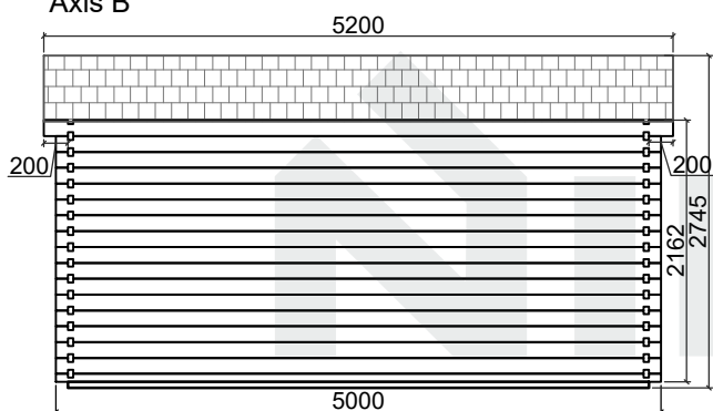
Axis B
