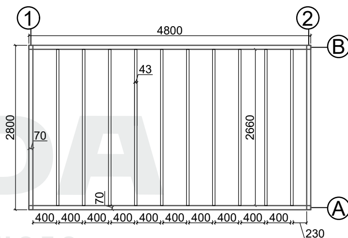
Base plan
