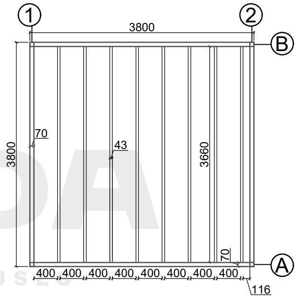
Base plan
