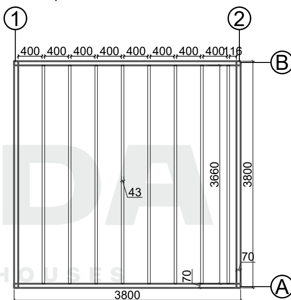
Base plan
