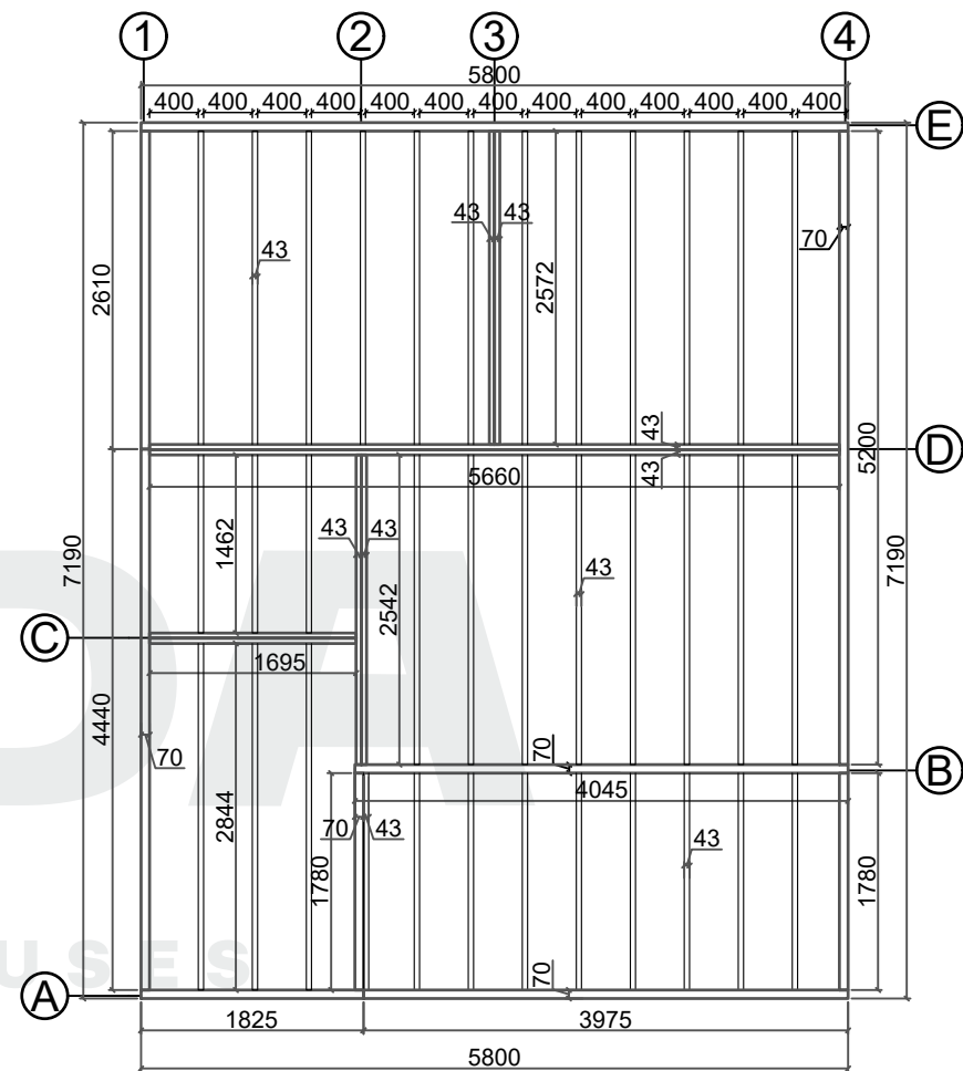
Base plan
