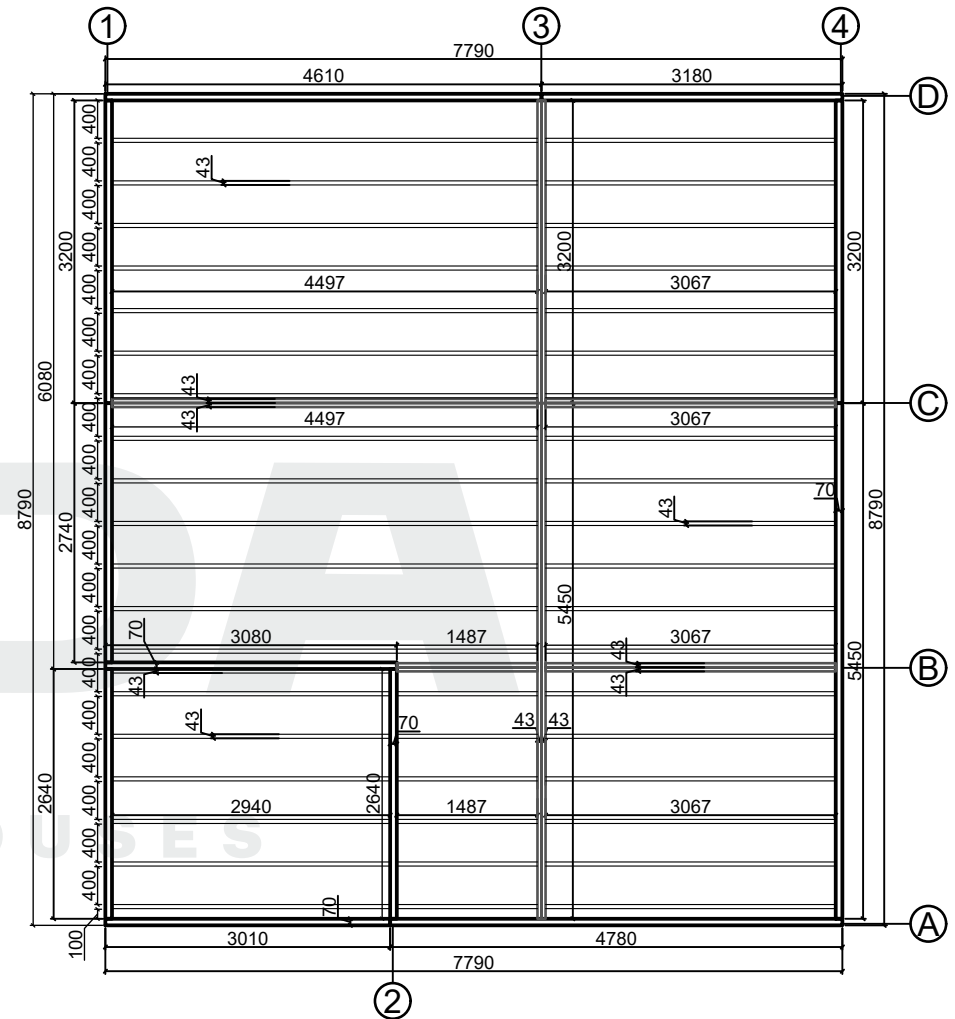
Base plan
