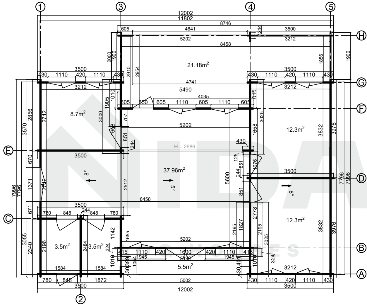
Floor plan
