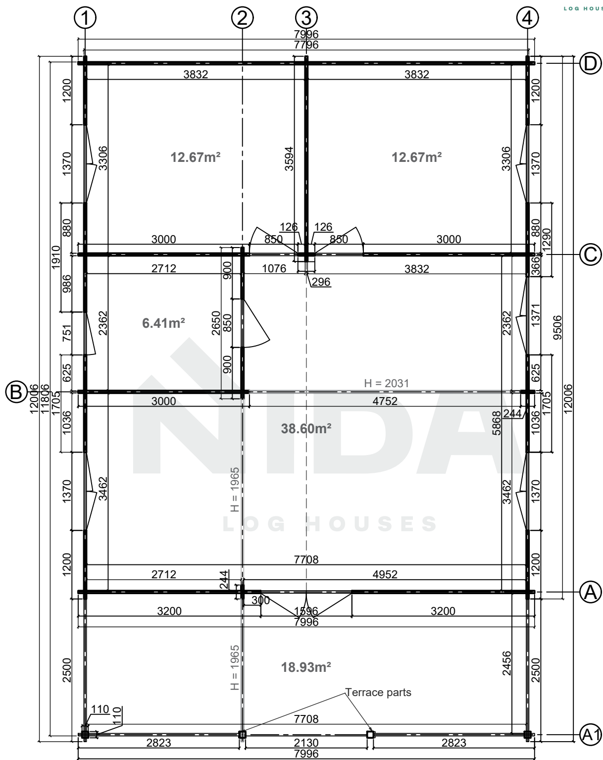
Floor plan
