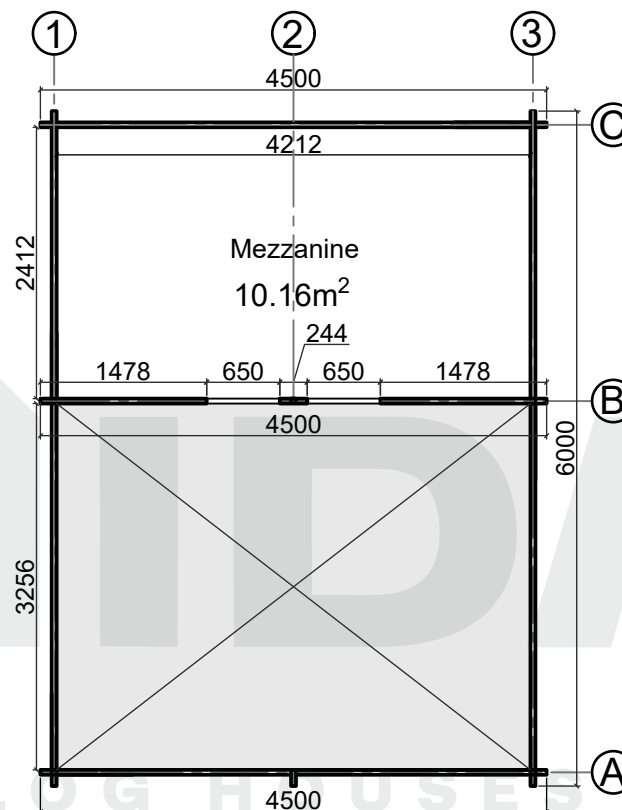
Mezzanine plan
