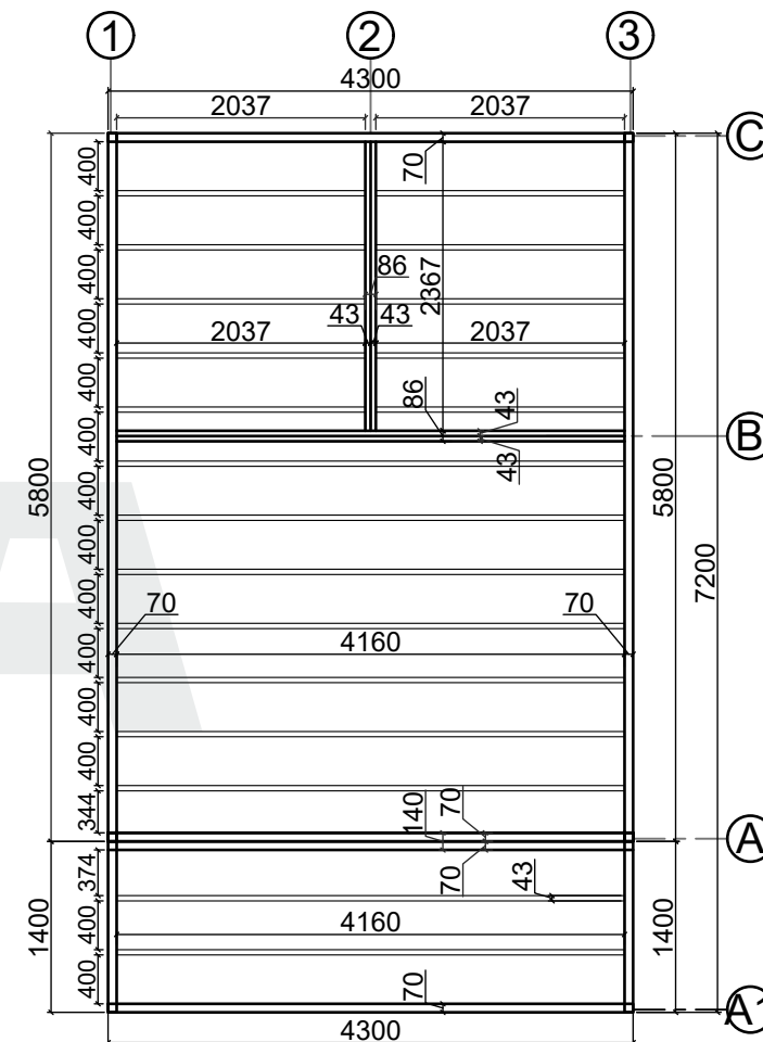
Base plan
