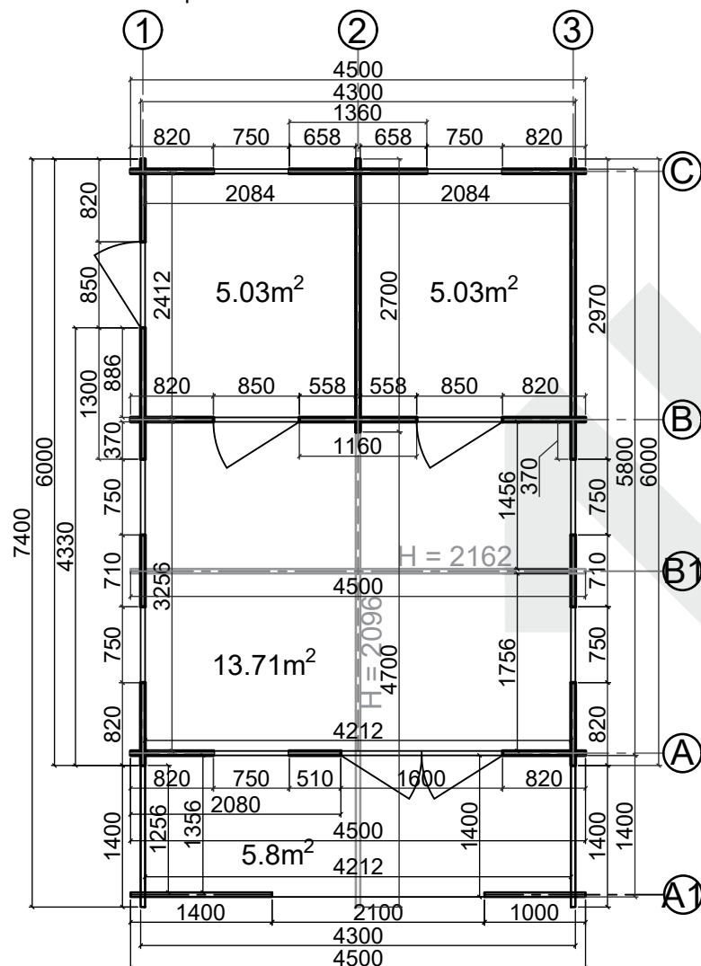
Floor plan
