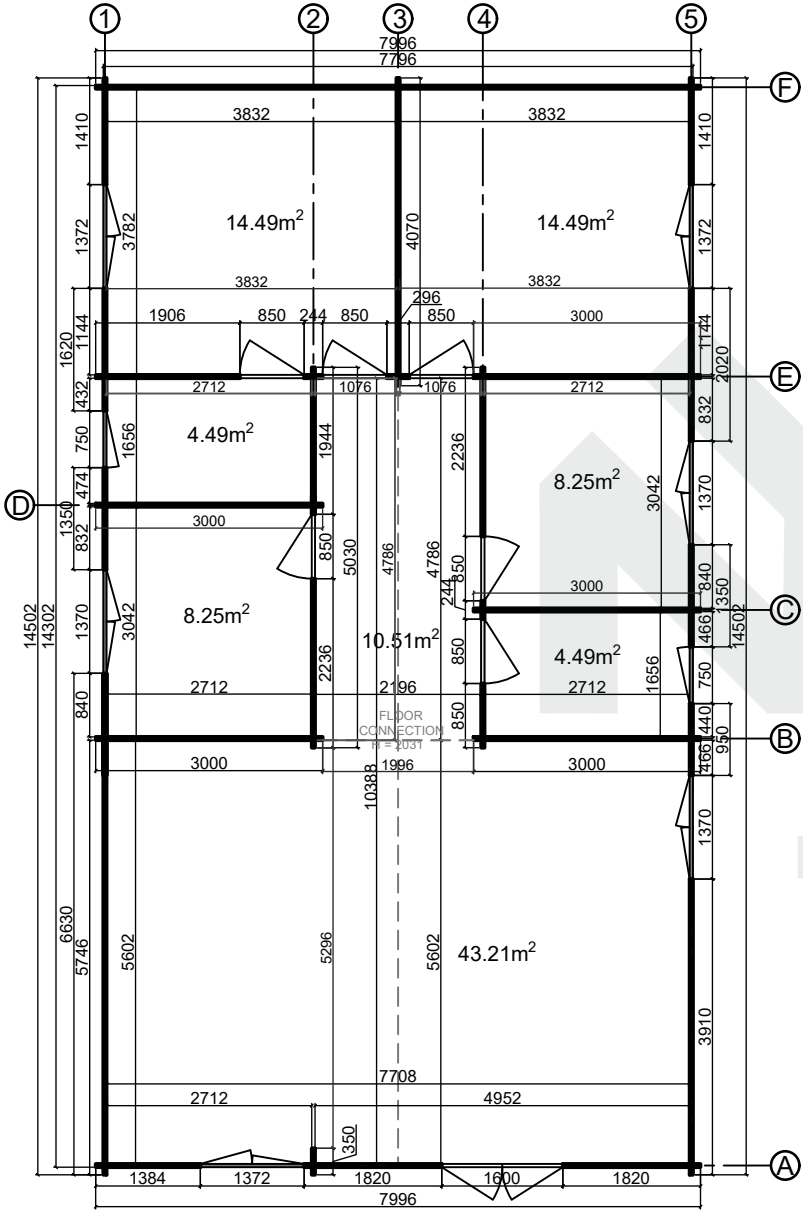
Floor plan
