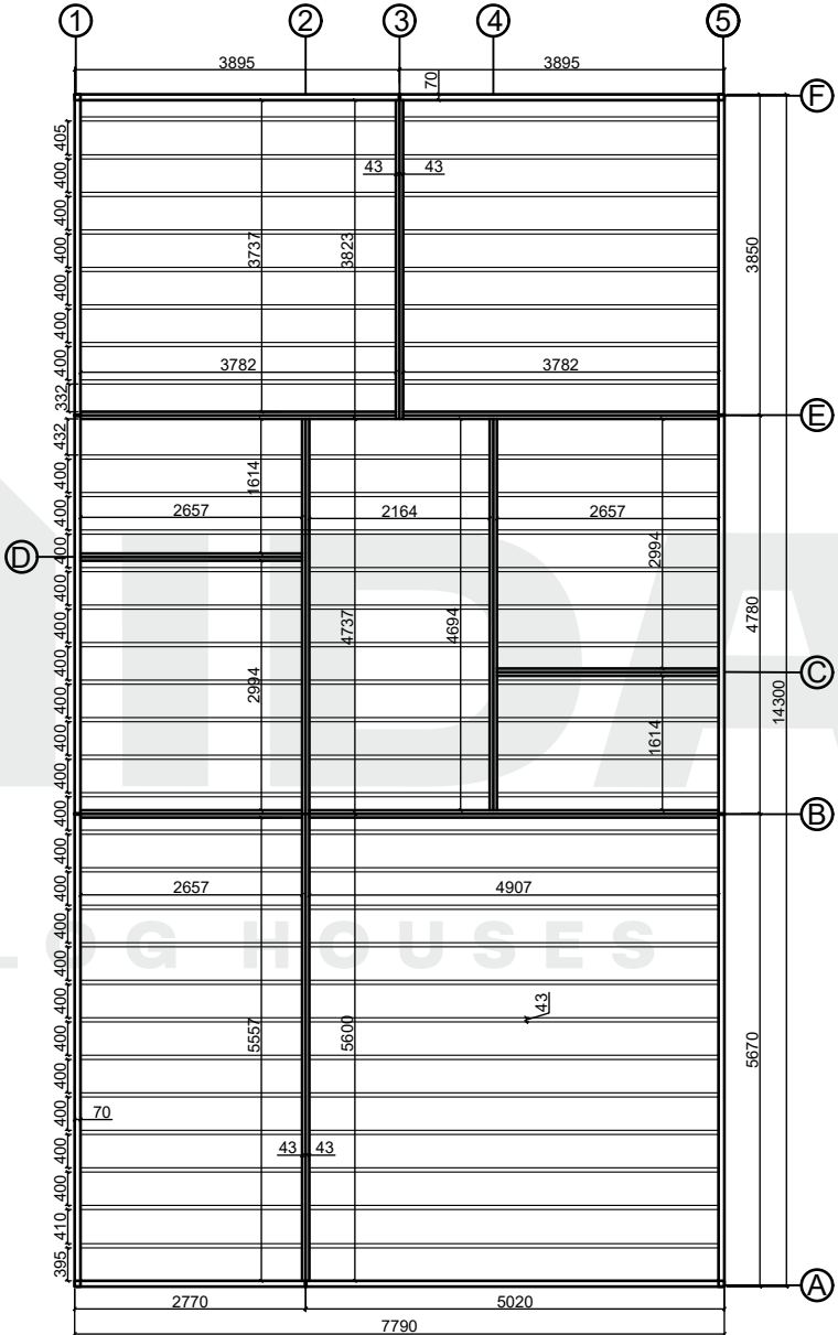
Base plan
