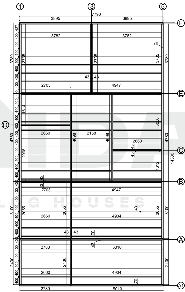
Base plan
