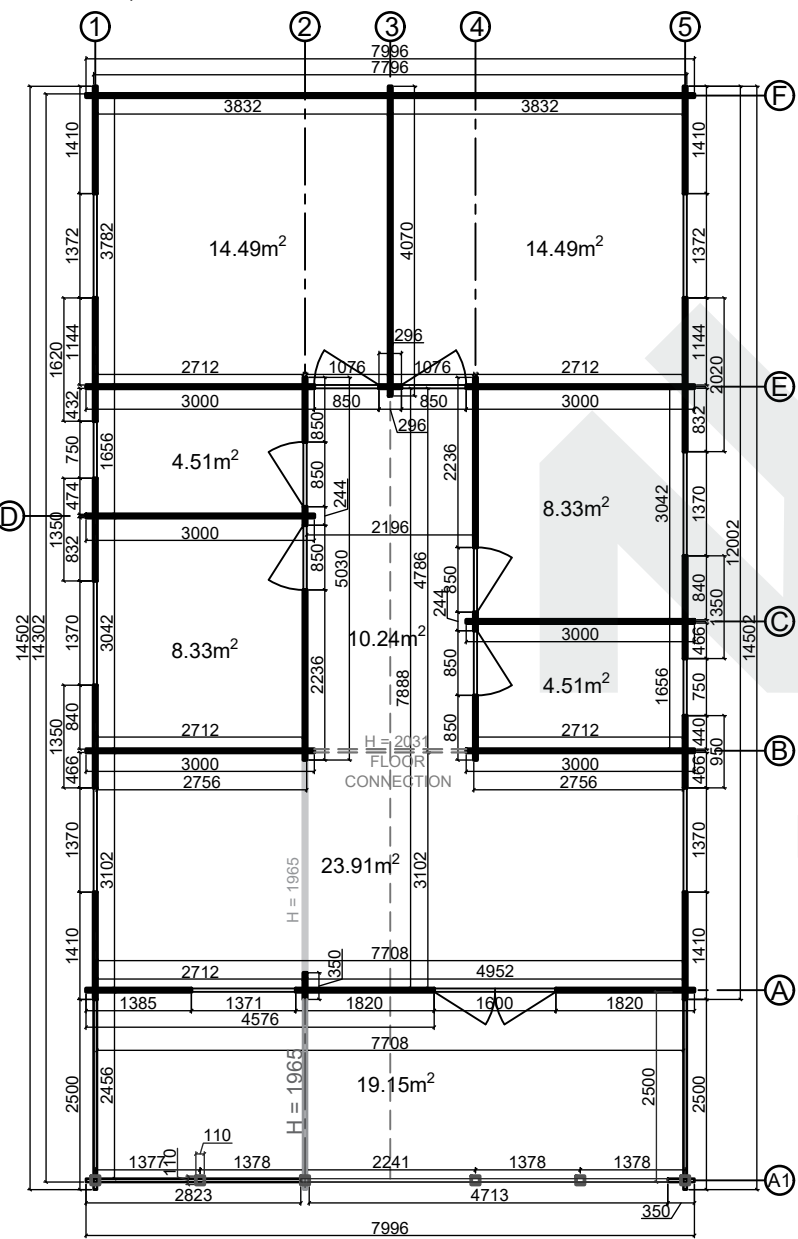
Floor plan
