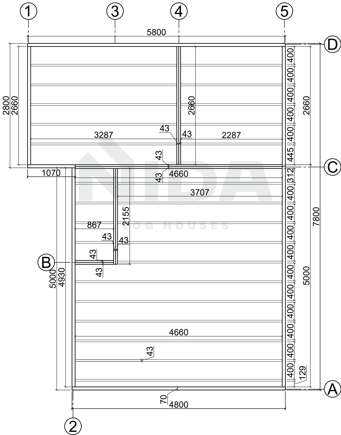
Base plan
