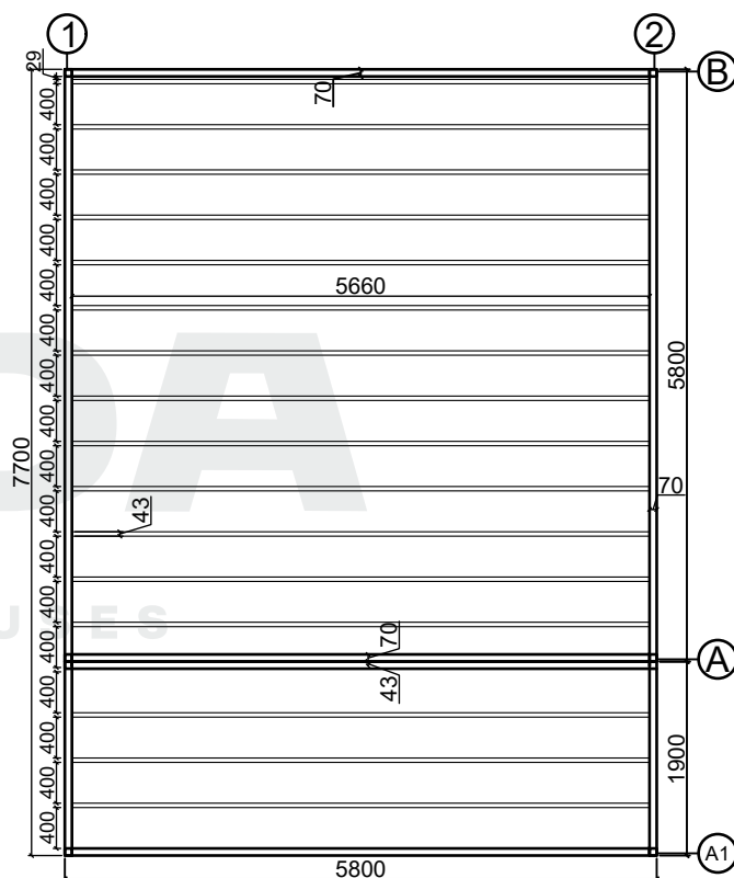
Base plan
