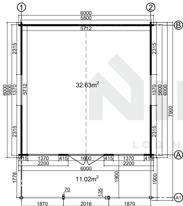
Floor plan
