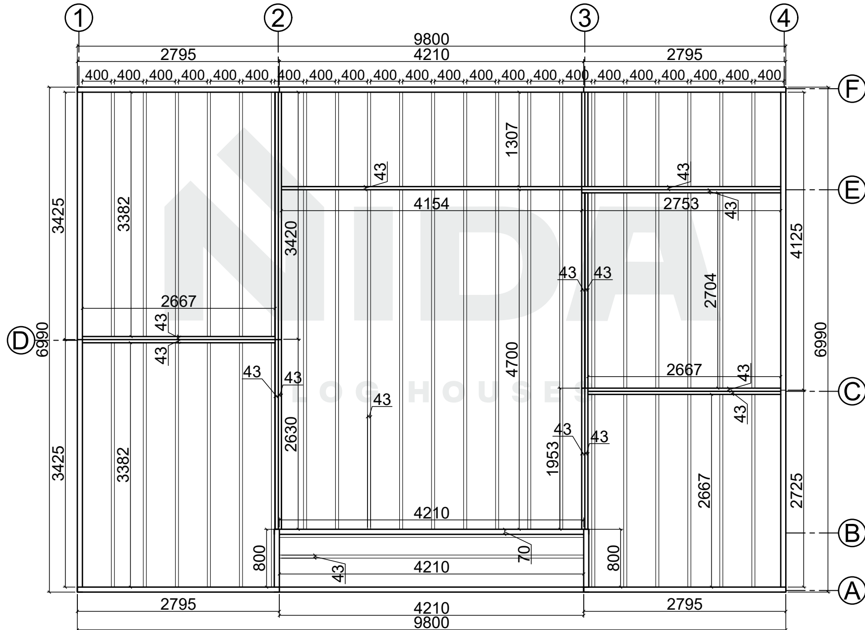
Base plan
