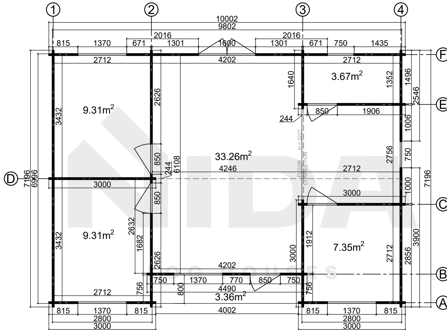
Floor plan
