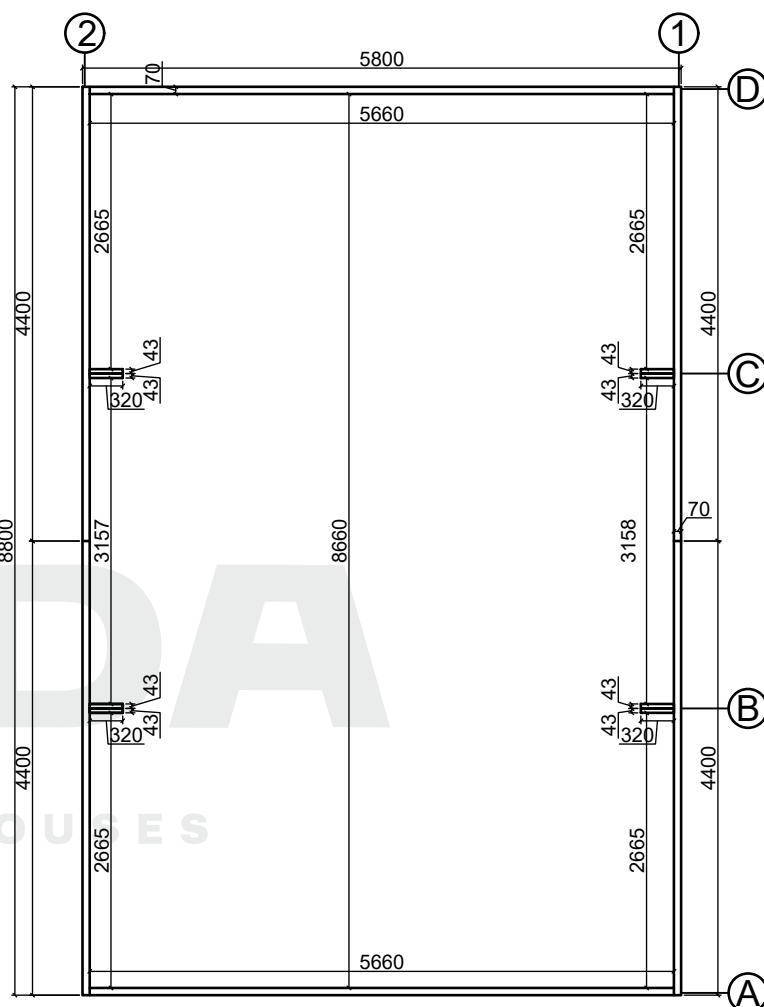
Base plan
