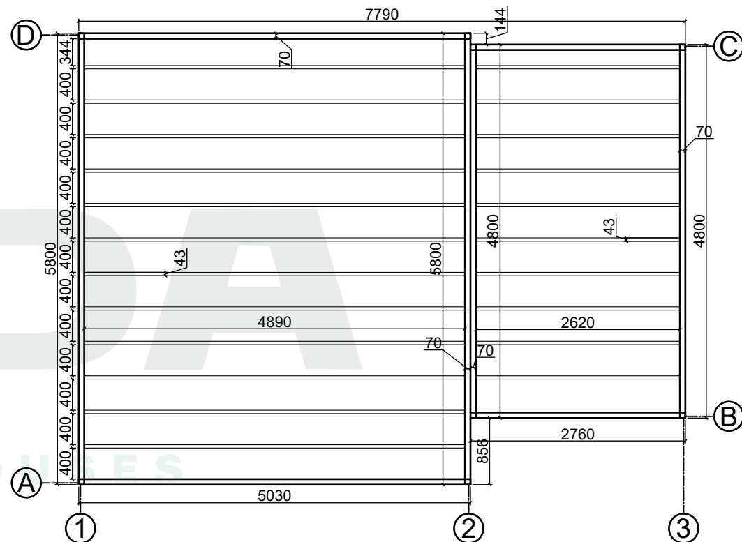
Base plan
