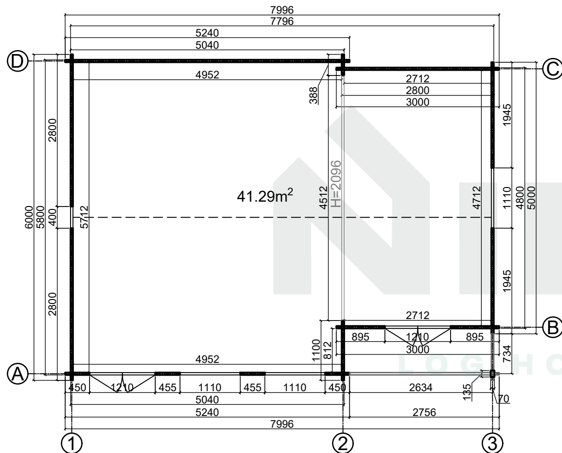
Floor plan
