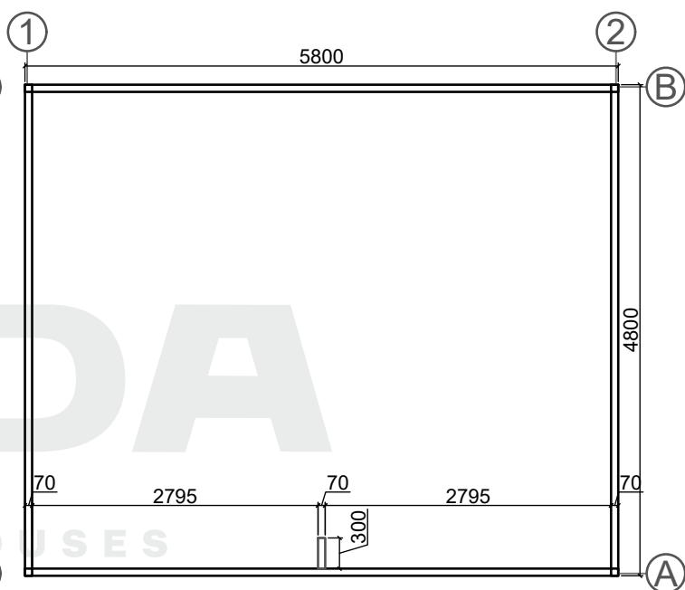
Base plan
