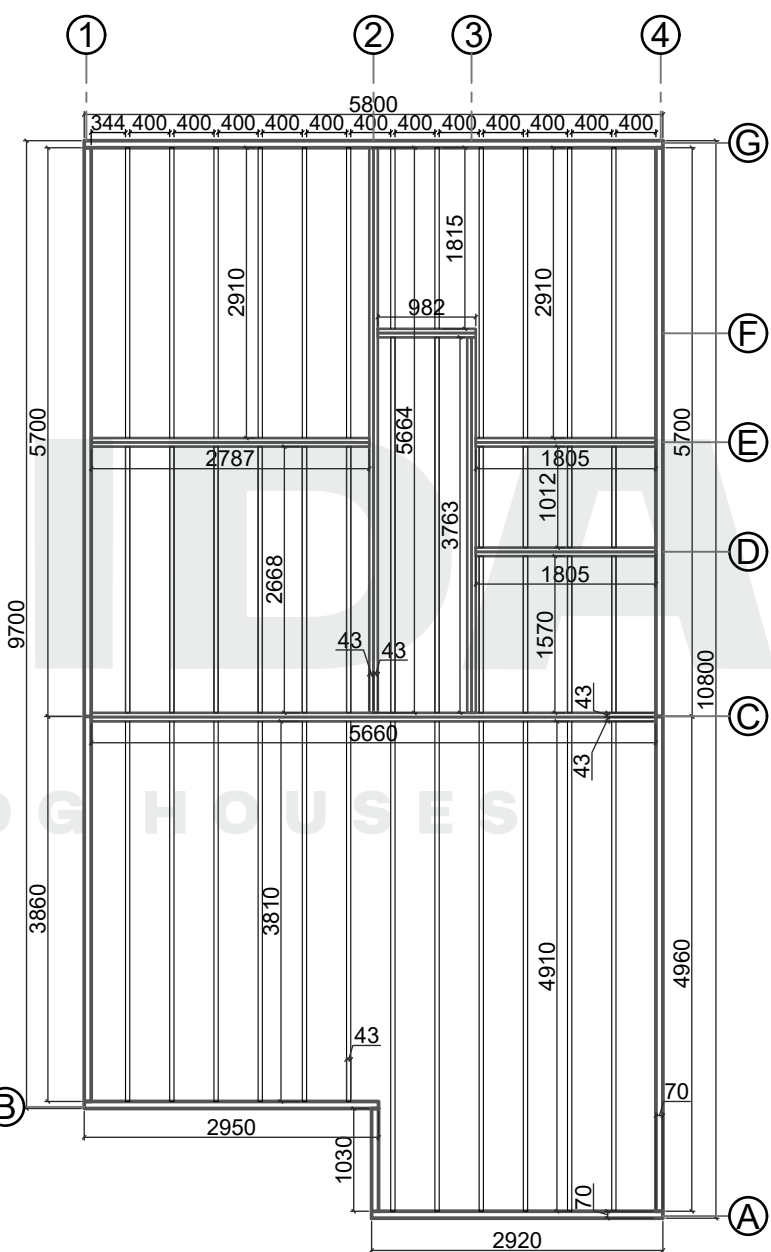
Base plan
