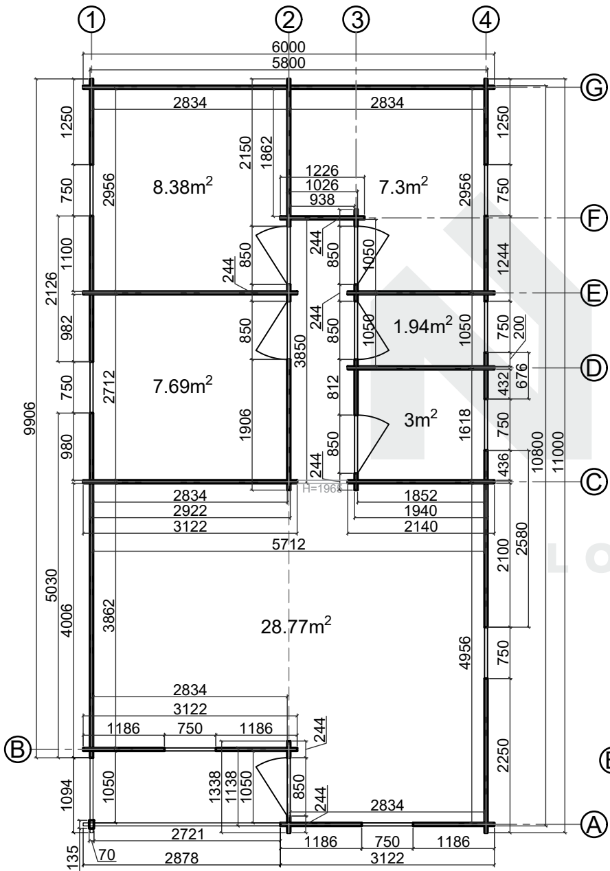
Floor plan
