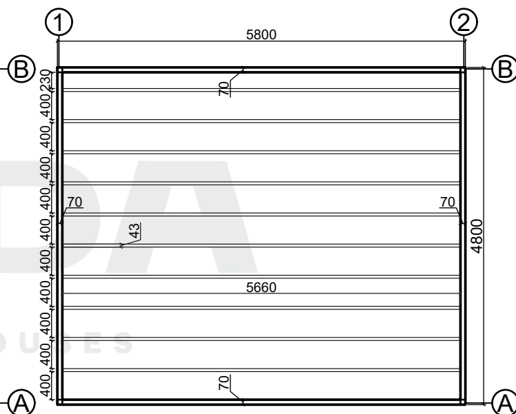
Base plan
