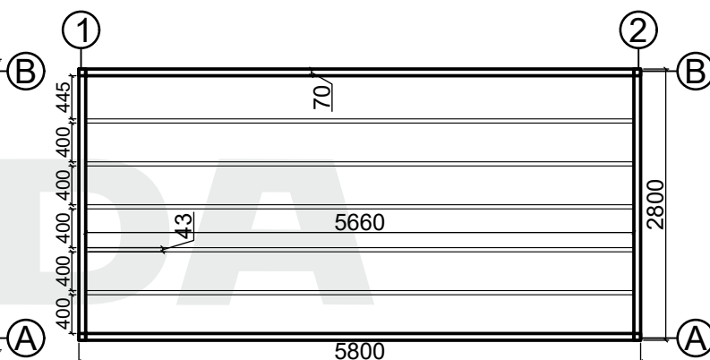
Base plan
