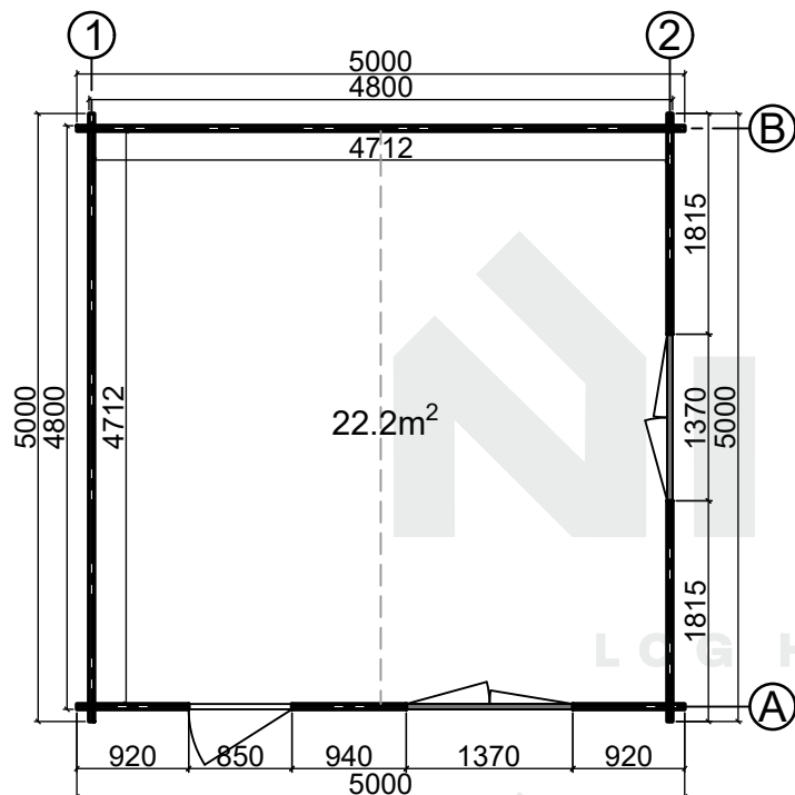
Floor plan
