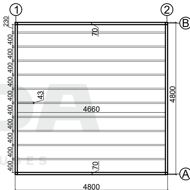
Base plan
