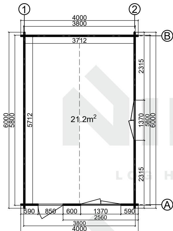
Floor plan
