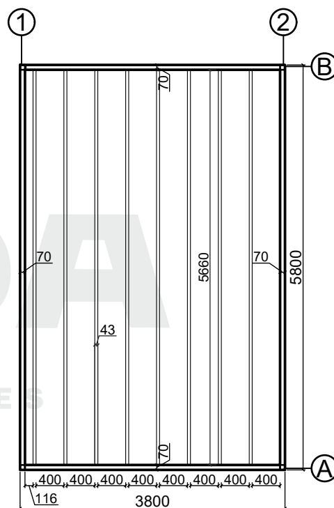
Base plan
