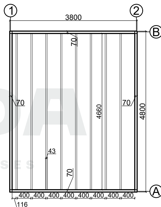
Base plan
