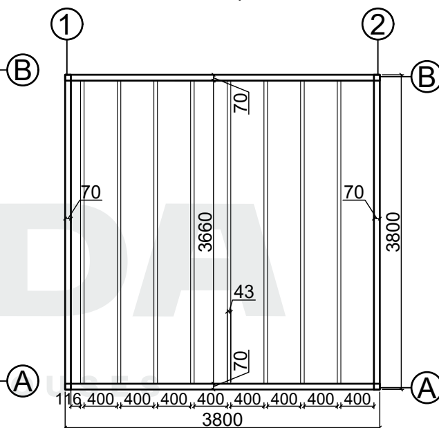
Base plan
