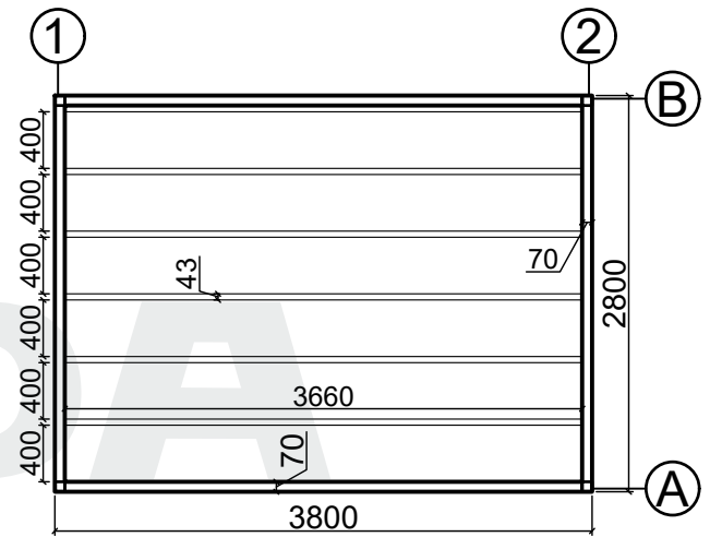
Base plan
