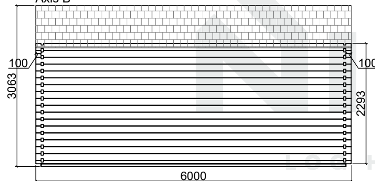
Axis B
