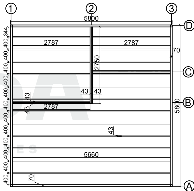
Base plan
