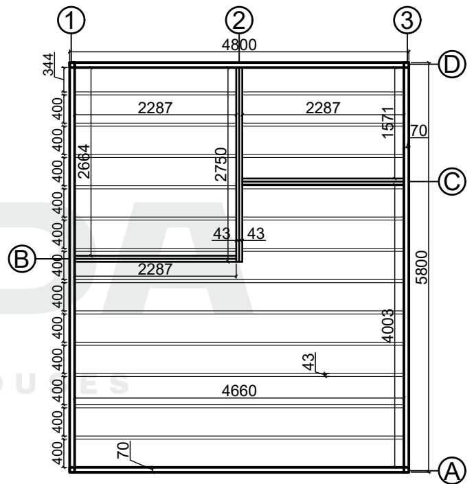
Base plan
