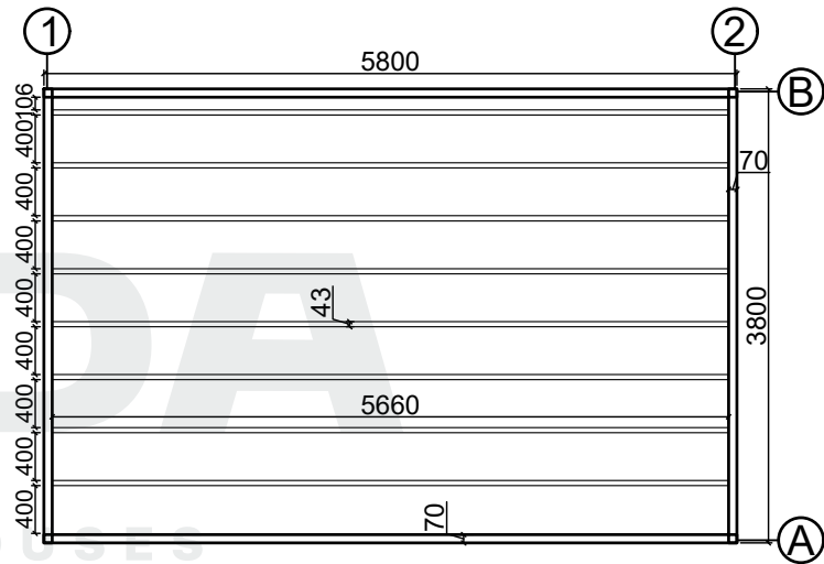
Base plan
