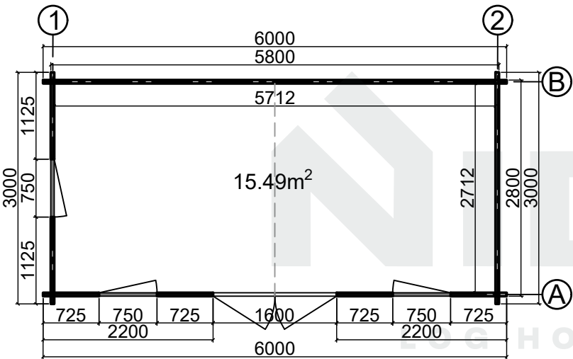
Floor plan
