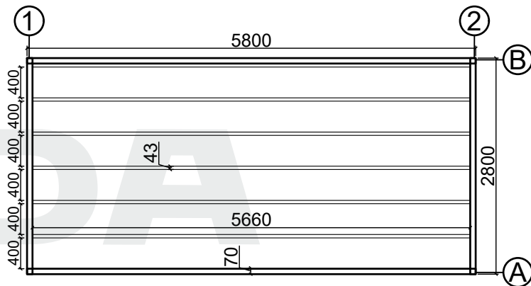
Base plan
