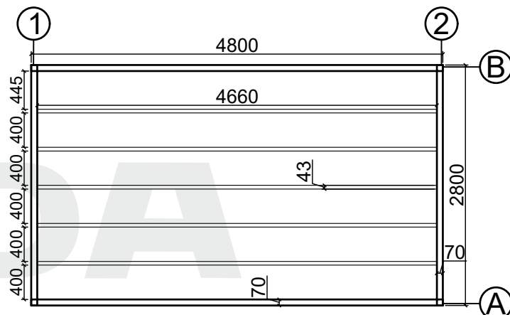
Base plan
