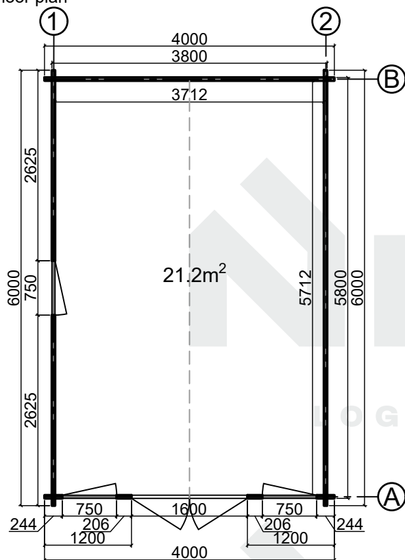
Floor plan
