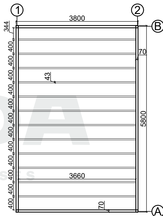
Base plan
