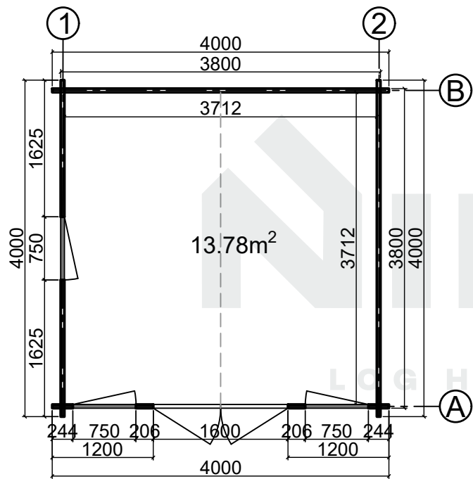
Floor plan
