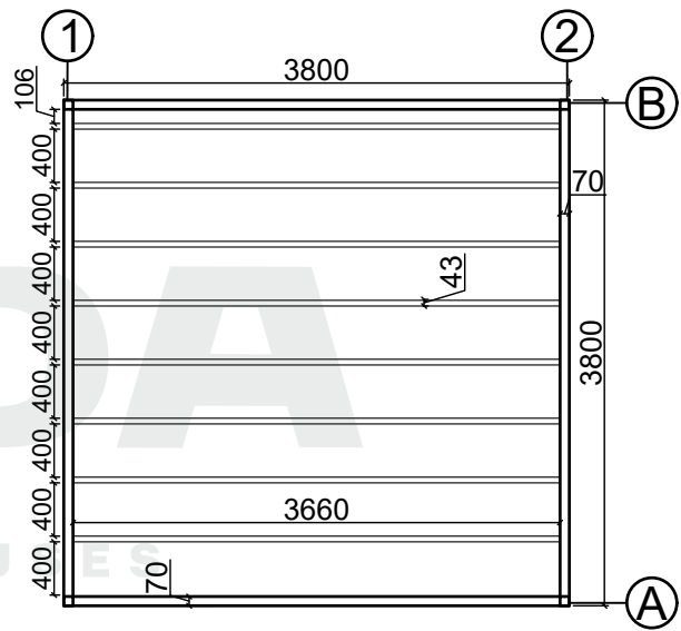
Base plan
