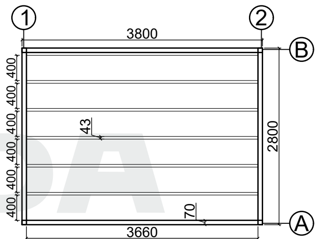
Base plan
