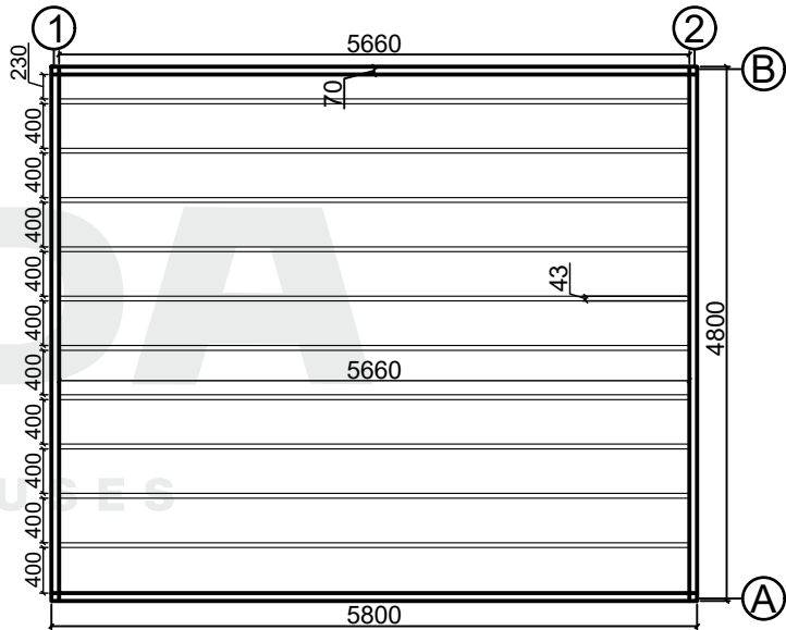
Base plan
