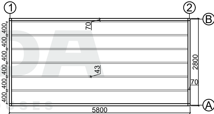
Base plan
